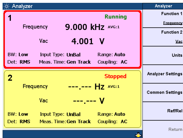
Figure 3-12 Voltage measurement
