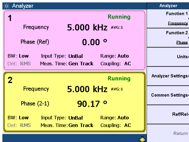
Figure 3-19 Phase difference measurement
