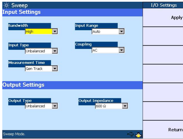
Figure 4-11 I/O settings configuration
