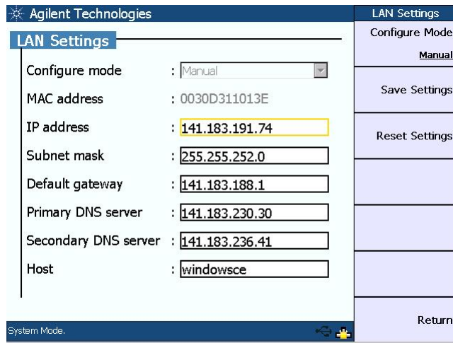
Figure 2-4 Manual configuration of the LAN settings
